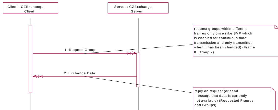
Figure 2: Sequence Diagram
