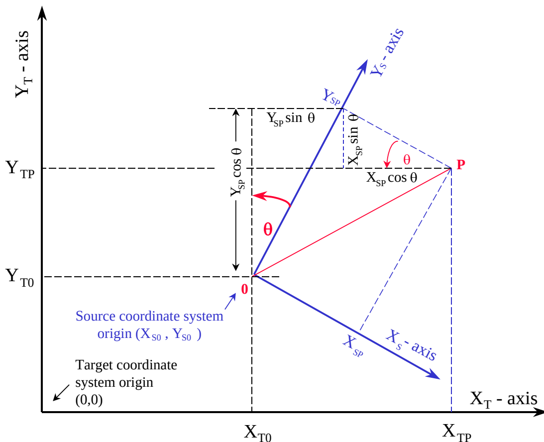
Figure 15 – Similarity Transformation
