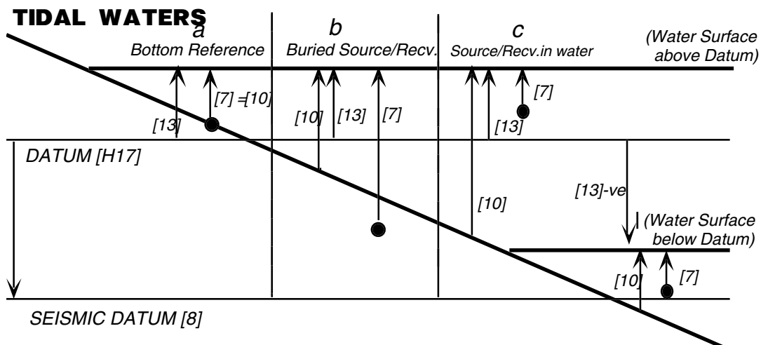
Figure 4. Tidal elevations
